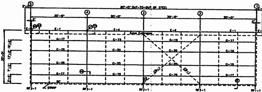
SIDEWALL FRAMING: FRAME LINE A
