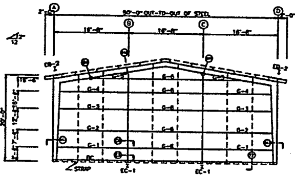
ENDWALL FRAMING: FRAME LINE 1
