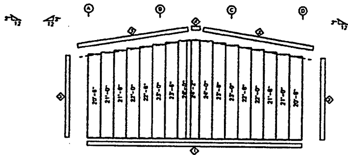
ENDWALL SHEETING & TRIM: FRAME LINE 1 PANELS: 26 Co. R - SLB'S Leather Brown
